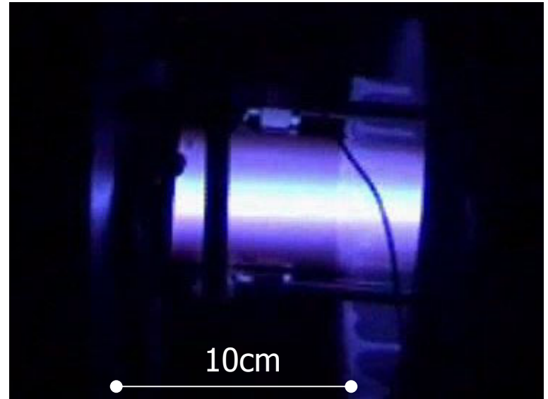
Argon
